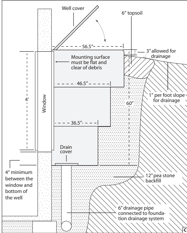
Side view of well installation
